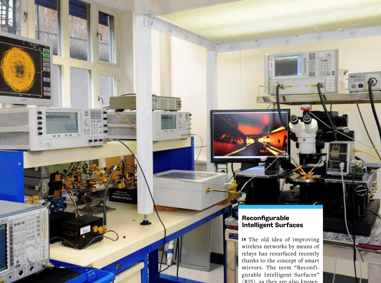
Millimeter waves source-pull/load-pull measurement platform
